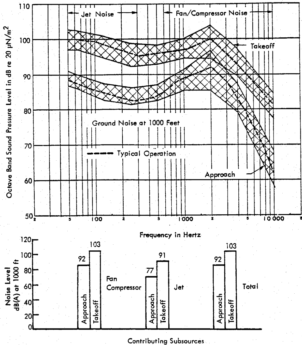
Figure 2.1-4. Noise Levels and Spectra of 4-Engine High Bypass Ratio Turbofan Aircraft
