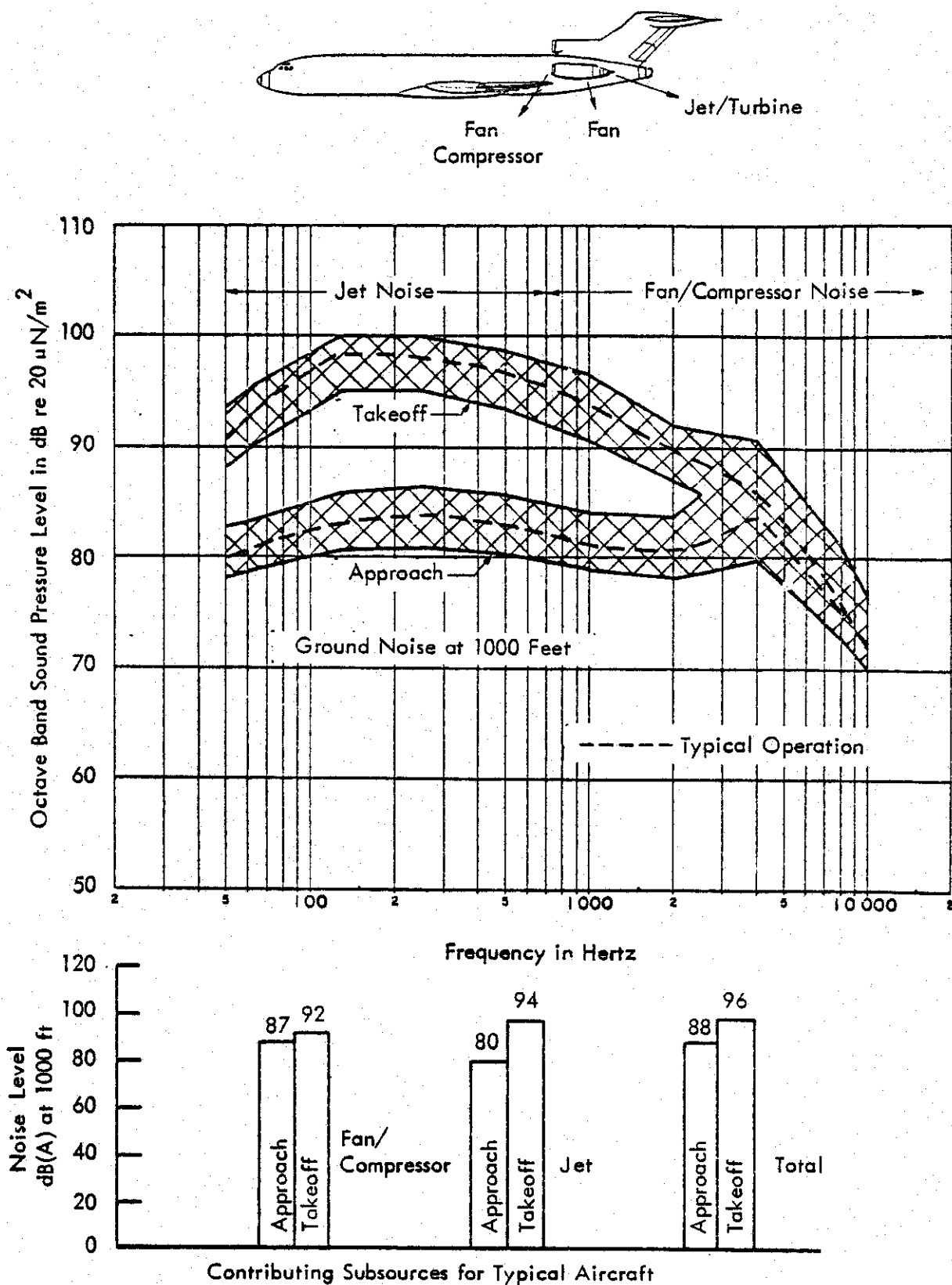
Figure 2.1-3. Noise Levels and Spectra of 2-3 Engine Low Bypass Ratio Turbofan Aircraft
