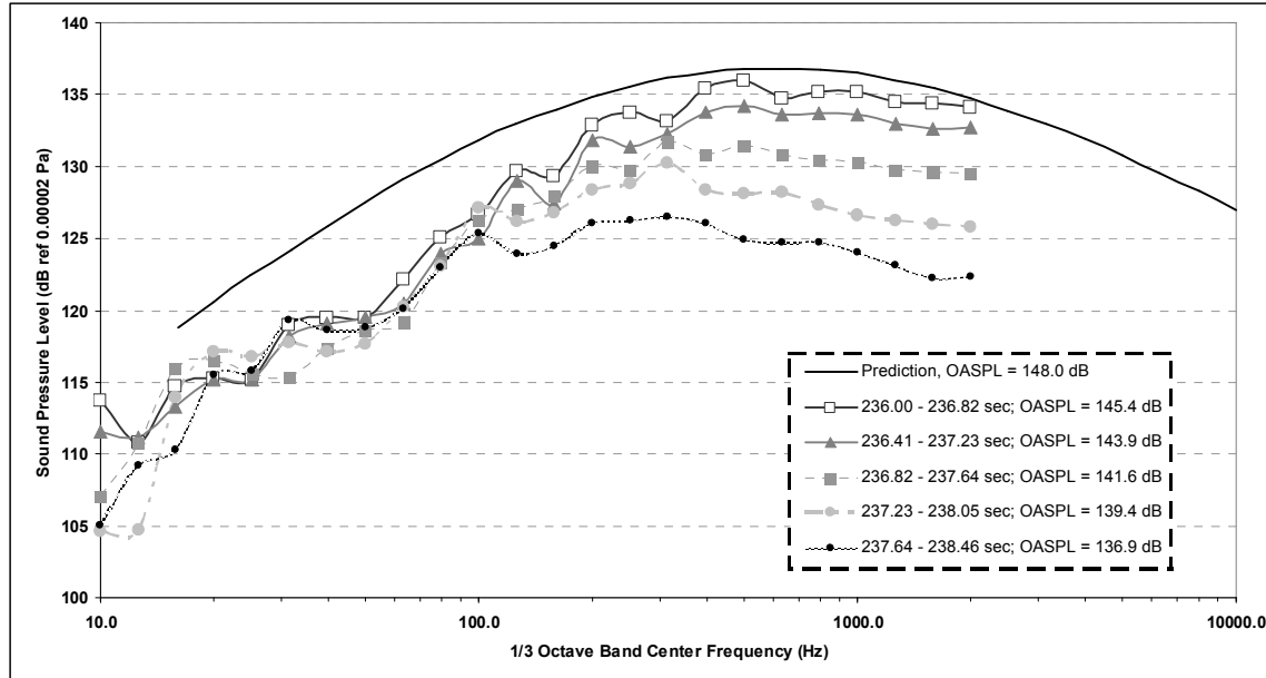
Figure 2. One-third octave and overall sound pressure level comparisons between the VAEPP method and the ALV-X1 measured data.
