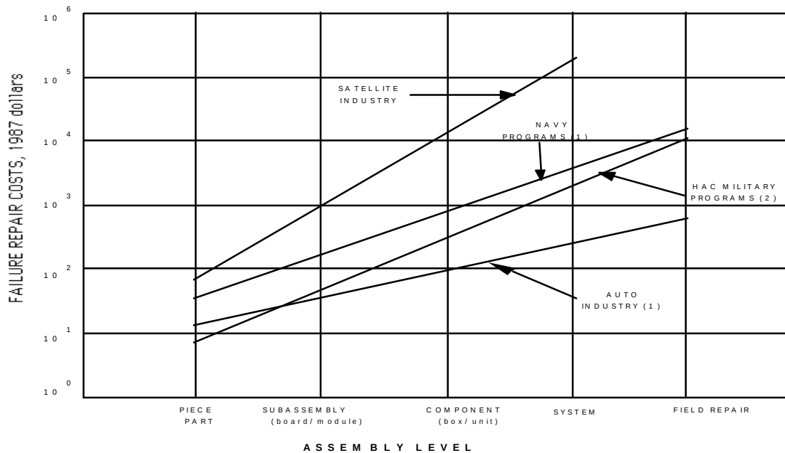
Figure 1 Hardware Failure Costs vs. Assembly Level
