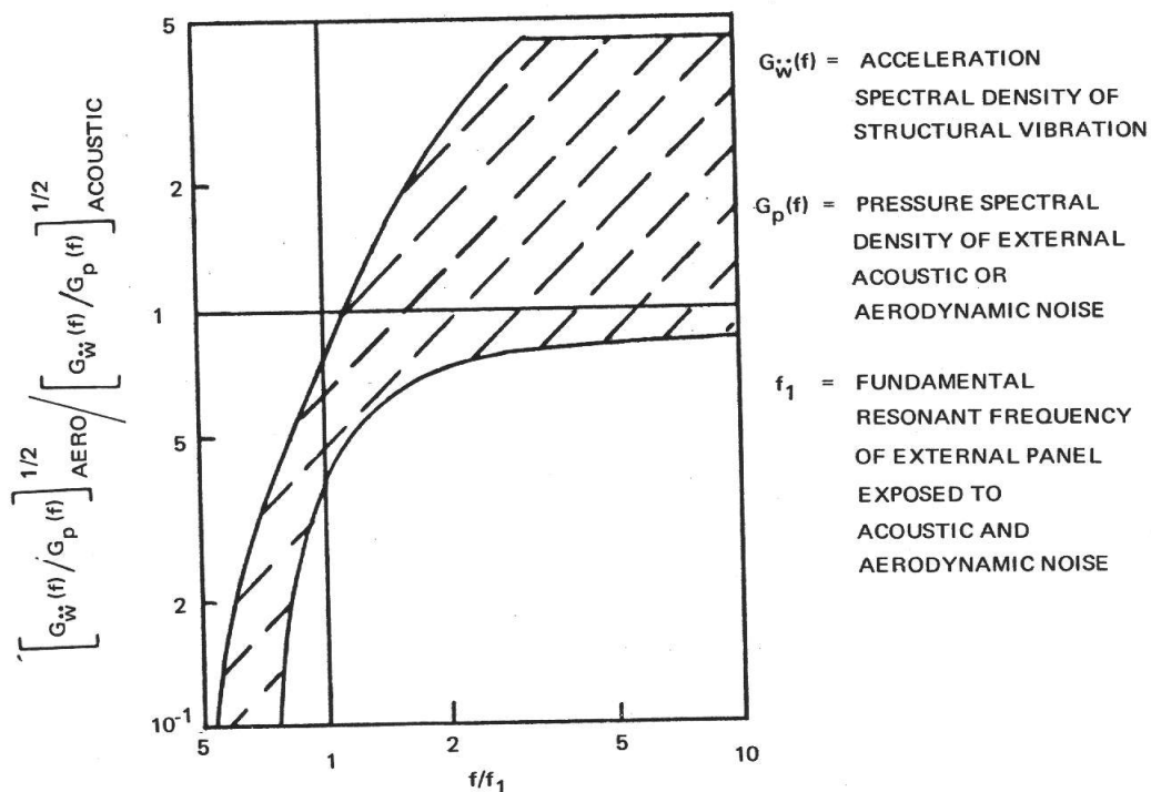
Figure 20. — Vibration efficiency of aerodynamic noise relative to acoustic noise.
