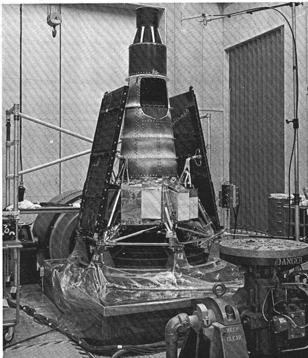
Figure 27.—Laboratory vibration test of the Ranger spacecraft.
