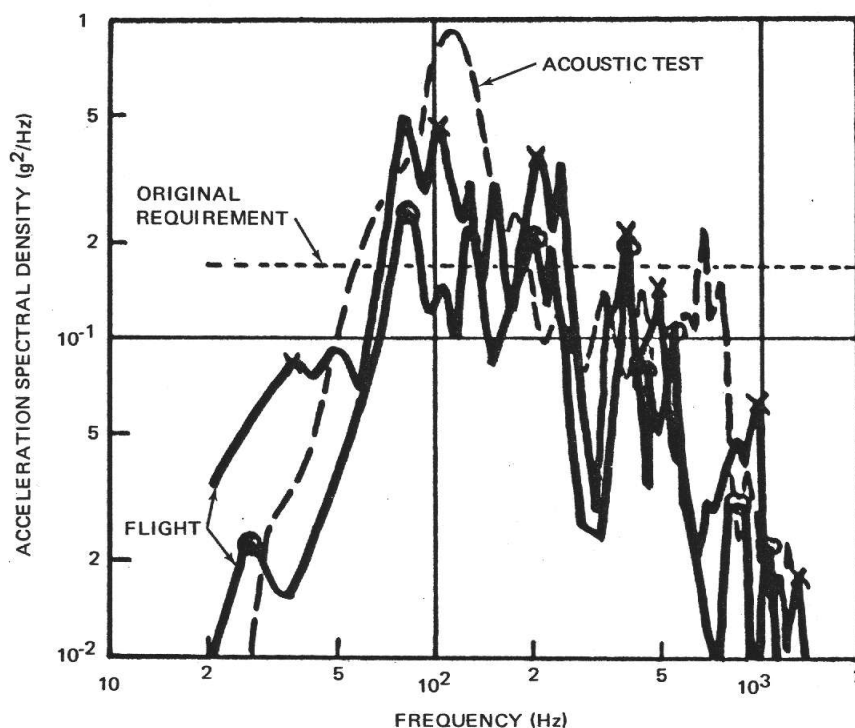
Figure 39.—Comparison of vibration spectra from acoustic test with flight and with original design and test requirement.
