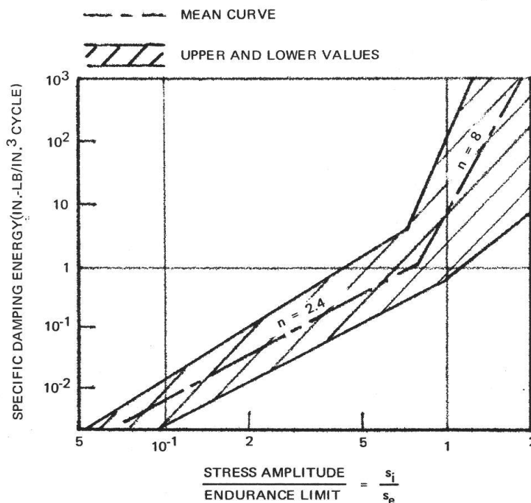
Figure 6.—Material-damping properties for various aerospace structures.
