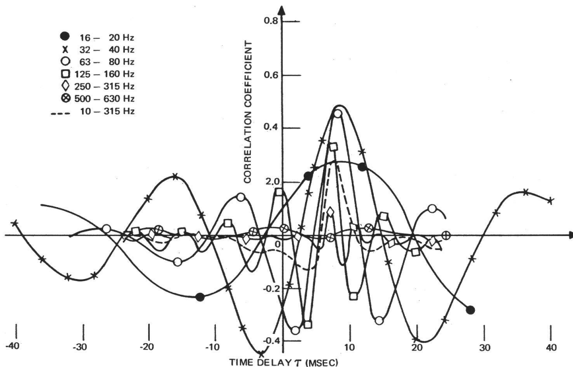
Figure 5.—Longitudinal cross-correlation of aerodynamic noise during the transonic period for two microphones located 40 in. apart on the external surface of the Apollo service module.
