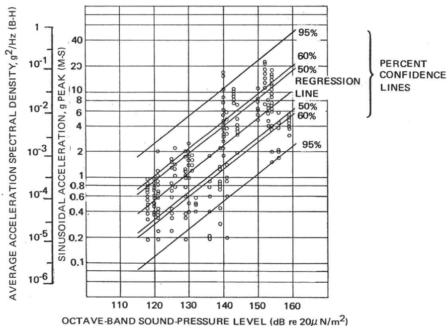
Figure 16.—Vibration-prediction curves for Mahaffey-Smith and Brust-Himmelblau methods in the 300- to 600-Hz octave band
