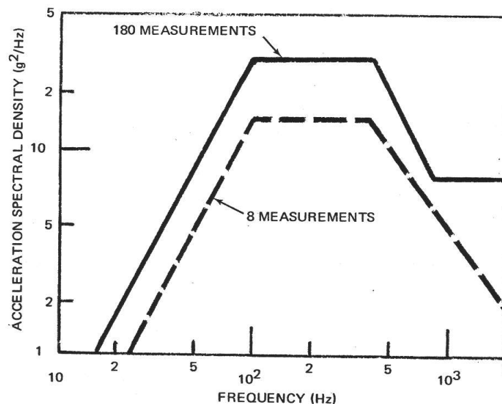
Figure 33.—Comparison of spectral envelope for 8 and 180 vibration measurements made on the external panels of the Apollo service module during acoustic testing.
