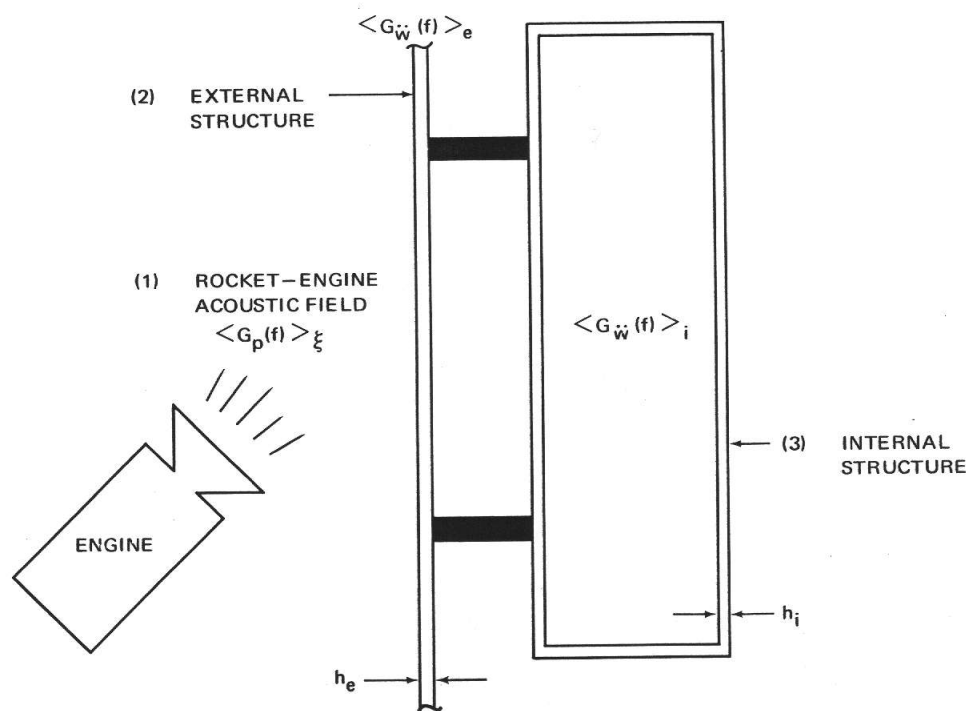
Figure 12.—Idealized representation of a simple space-vehicle structure used for predicting the space-average response of external and internal structure at higher frequencies by statistical-energy analysis.
