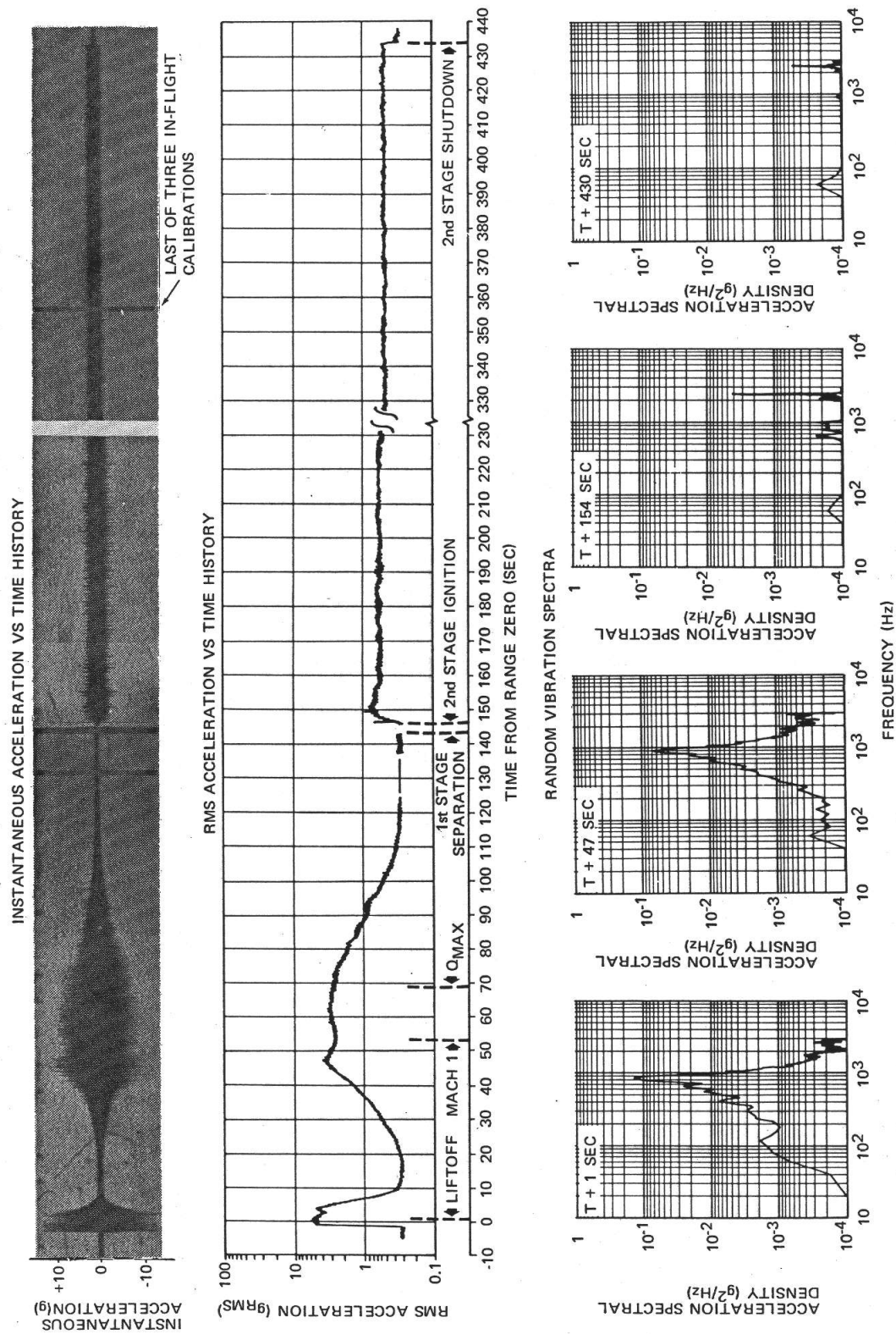
Figure 1.—Vibration measured on the S-IVB stage of the uprated Saturn I space vehicle during Apollo-Saturn flight SA-203.
