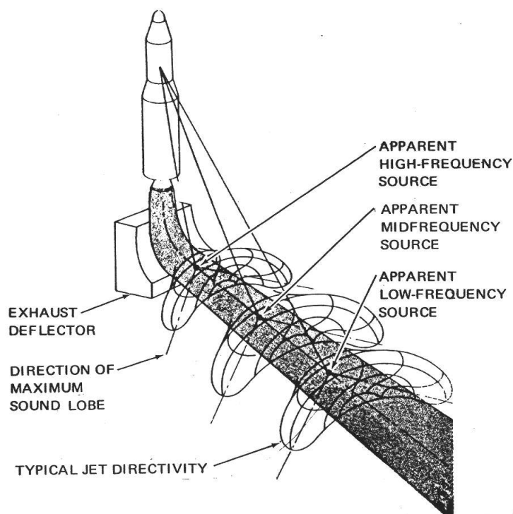
Figure 2.—Rocket-engine acoustic noise sources and directivity patterns to the space vehicle during liftoff or static firing.
