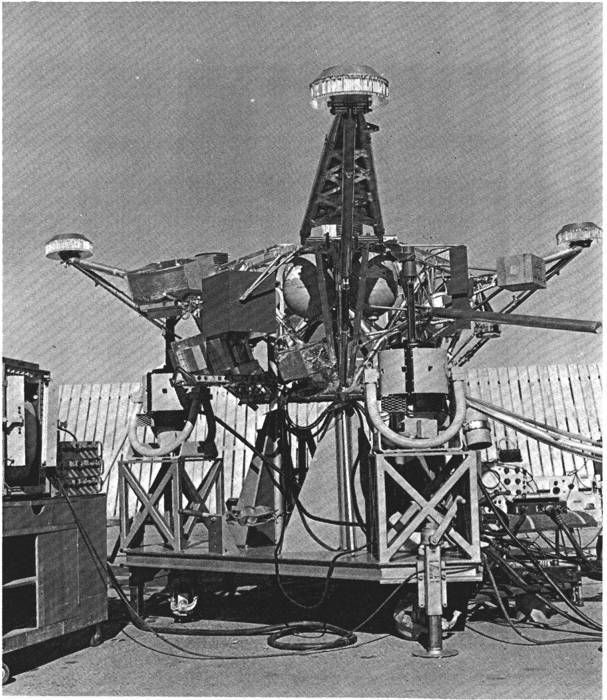
Figure 29.—Laboratory vibration test of the Surveyor spacecraft.
