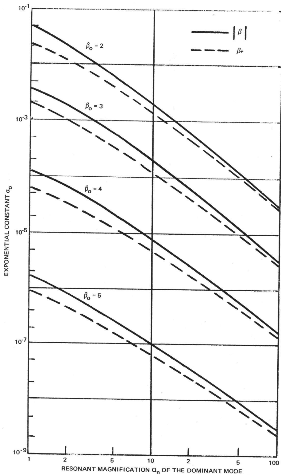
Figure 11. — Plot of exponential constant a_0 to be used in determining threshold-crossing probability.
