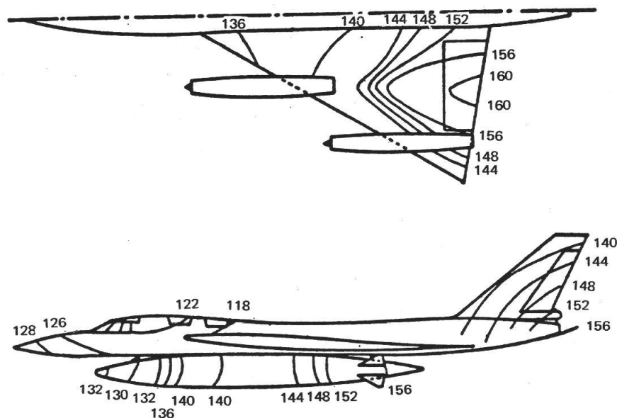
Figure 15.- Sound-pressure-level contours for the B-58 in the 300- to 600-Hz octave band.
