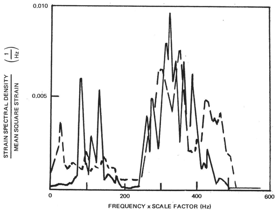
Figure 24. — Comparison of Apollo boilerplate service module vibration-strain spectra.
