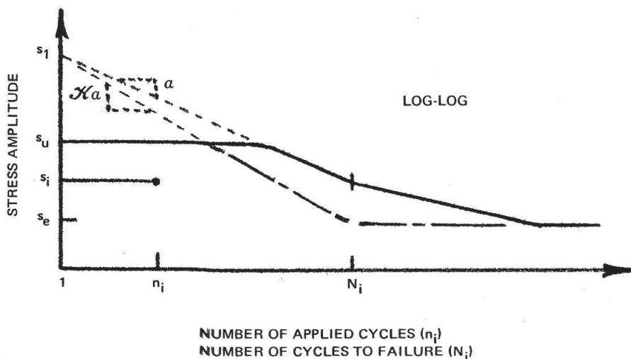
Figure 8.—Fatigue curve for a typical aerospace material under sinusoidal loading.
