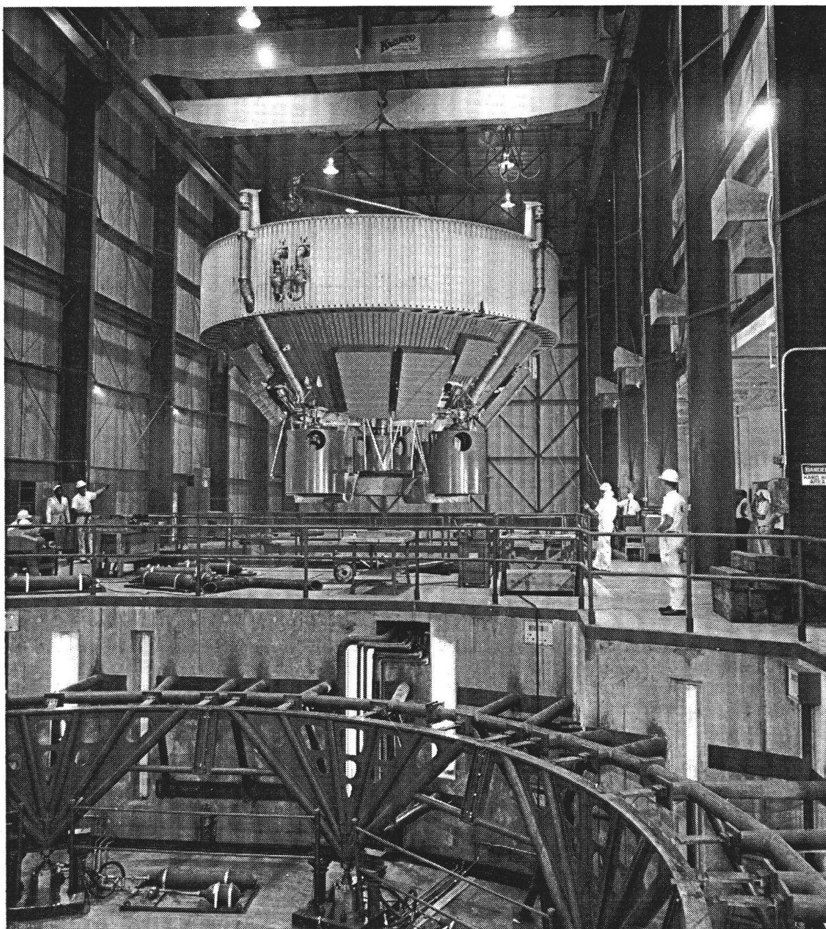
Figure 30.—Laboratory vibration-test facility of the thrust structure and aft skirt of the S-II stage, Saturn V launch vehicle.
