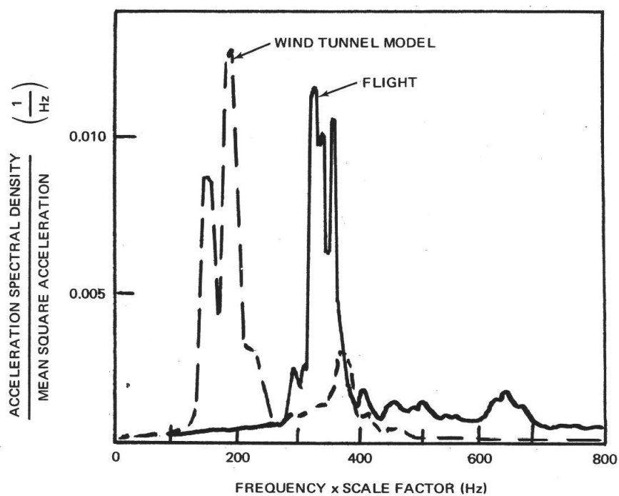
Figure 25. — Comparison of Apollo boilerplate service module vibration-acceleration spectra.
