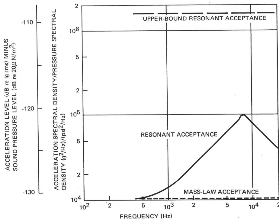
Figure 13. — Space-average acoustic acceptance for an idealized representation of space-vehicle external structure.
