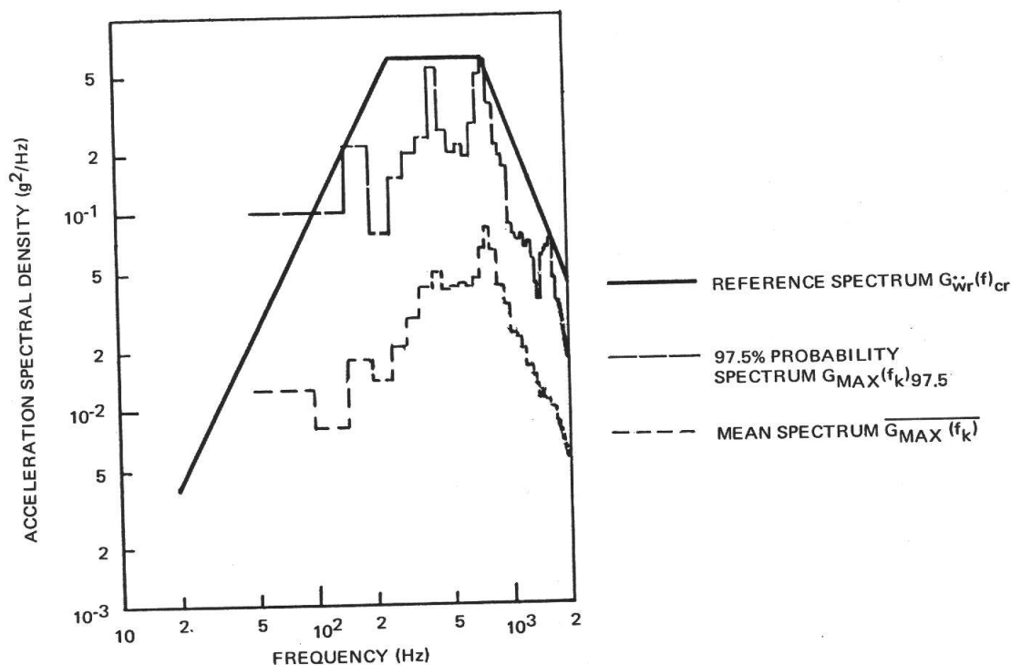
Figure 21. — Vibration-reference spectra for Barrett method on 50 flight measurements on the aft skirt of Saturn I fuel tanks.
