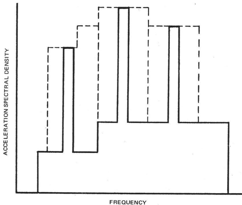
Figure 35. — Random vibration-test spectrum consisting of high-level narrow band "spikes" superimposed on lower-level wideband spectrum.
