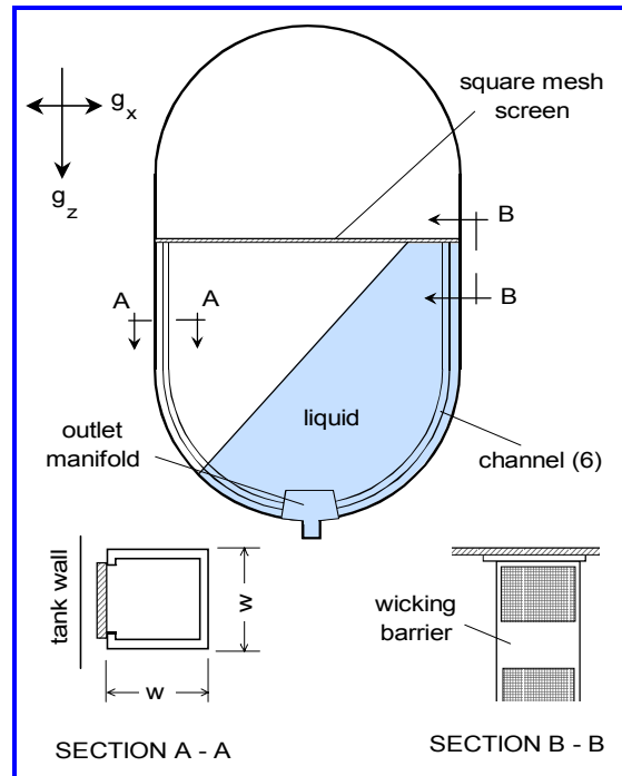
Figure 4.37. Schematic of channel PMD
