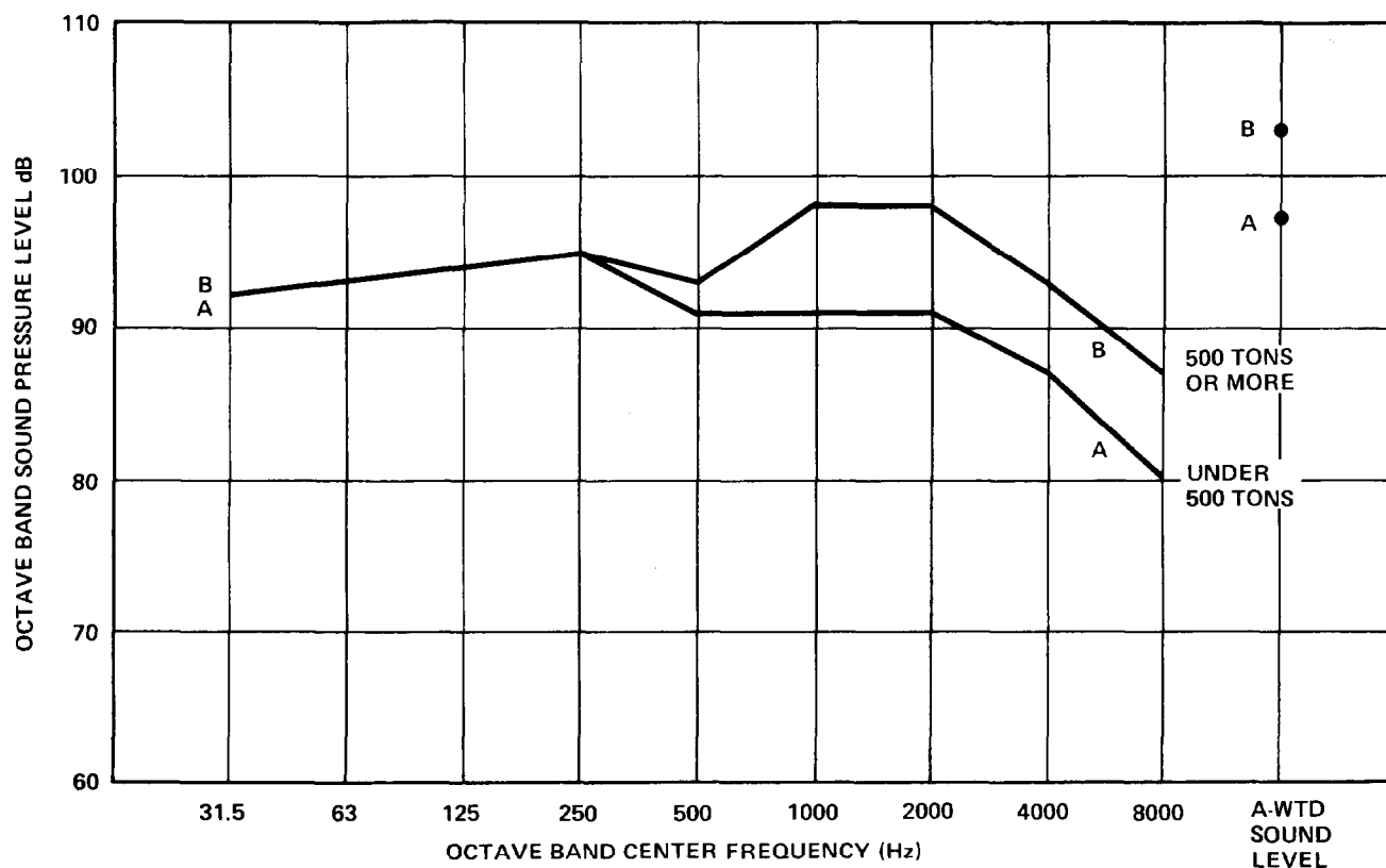
Figure C-2. Sound Pressure Levels of Centrifugal Compressors at 3-ft. Distance.
