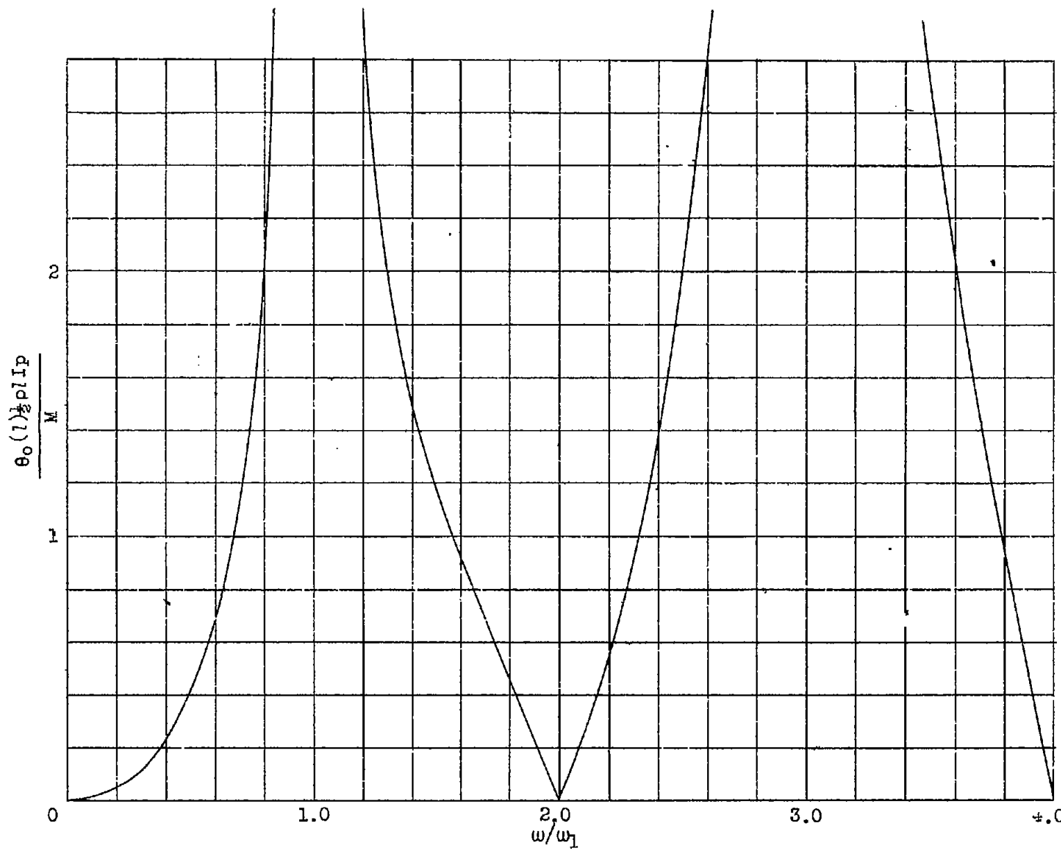
Figure 3.- Response curve for torsional vibration of a uniform beam.
