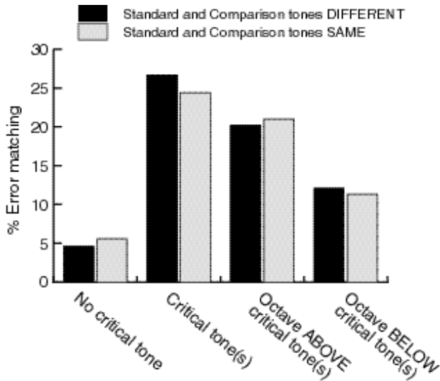
Figure 7: Octave generalization demonstrated by interference with pitch memory. Two tones are presented, subjects are asked whether they are the same or different, and the fraction of errors is recorded. Other ‘interfering’ tones are presented between the standard (target) and comparison tones, lowering the fraction of correct responses. When an interfering tone matches the target tone, subjects make more mistakes in pitch memory; the same holds for the octaves of the target tone, but more so for an octave above than for an octave below (from Deutsch 1973).
