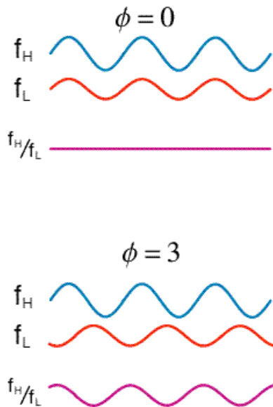
Figure 9: Demany and Semal's stimulus for measuring pitch fusion. Two tones, high and low (blue and red) are modulated in frequency and presented to different ears. As the relative phase ( \phi ) between the frequency modulation changes, so does the interval between the two tones (purple).
