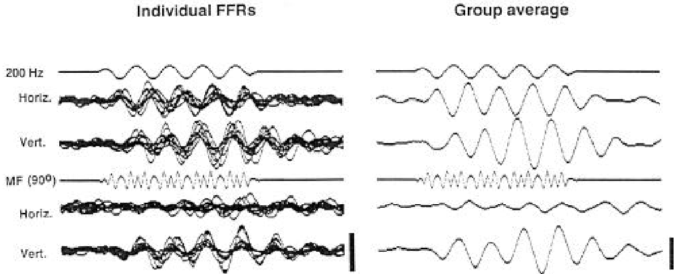
Figure 5: Electroencephalogram (EEG) of Frequency Following Response (FFR) to pure tone and missing fundamental stimuli. From top to bottom, traces are: pure-tone stimulus waveform, horizontal and vertical current dipole responses, a missing fundamental (MF) stimulus of three harmonics with one component 90° out of phase with the others (for minimum amplitude modulation), and horizontal and vertical current dipole responses. EEGs from horizontal current dipole correspond to auditory nerve fibers; those from vertical dipoles correspond to brainstem activity. Vertical bars represent 0.5 \mu V for individual and 0.25 \mu V for group FFRs; horizontal dimension shows 50 msec of time. Note that the vertical current dipole response to the missing fundamental is larger than the horizontal response (from Galbraith 1994).
