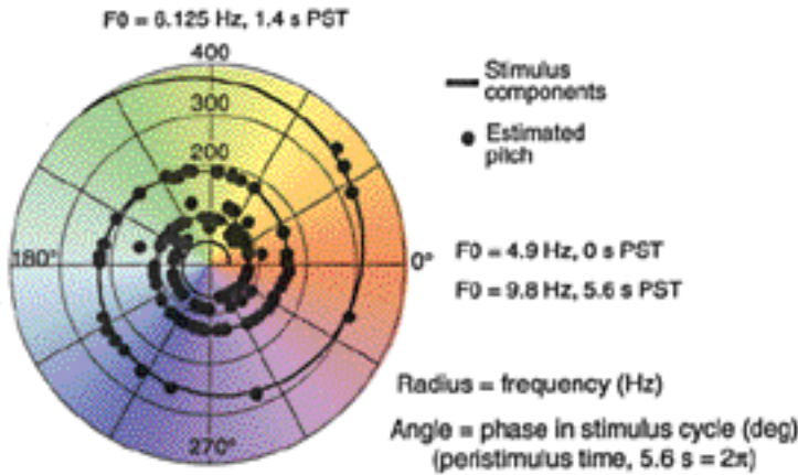
Figure 8: Cariani and Delgutte's algorithm (1996) predicts subharmonic pitch mistakes. Dots represent pitches estimated as the most common interspike interval in pooled recordings from cat auditory nerve fibers, when stimulated by Shepard tone complexes composed of all octaves of a given pitch. The color represents the pitch chroma on which the tone is based. The black spiral line represents frequency components physically present in the stimulus. Most estimated pitches lie on this line. Those that do not lie instead on another spiral (not drawn) which corresponds to the second subharmonic of one of the frequency components, which is not present in the stimulus.
