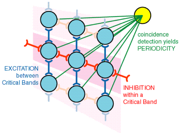
Figure 6: Neural networks for calculating the missing fundamental or periodicity of a stimulus. Frequency-tuned neurons (cyan circles) in the inferior colliculus are arranged in bands of similar tunings (light magenta). Connections are inhibitory (red) within a layer, and excitatory (blue) between neighboring layers. A coincidence detector (yellow) receives input (green) from nearby neurons and then fires with periodicity of the stimulus waveform.
