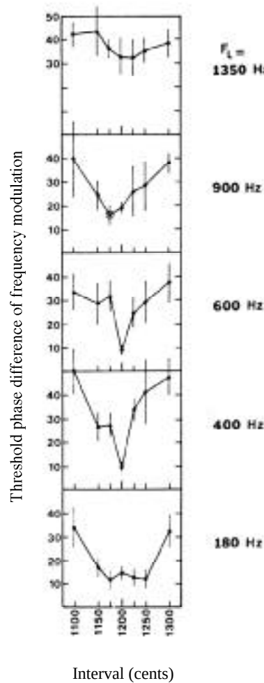
Figure 10: Improved pitch fusion for octave-related tones, measured by just-noticeable phase difference between high and low frequency modulated tones. Frequency to right is that of lower frequency (from Demany and Semal 1990).
