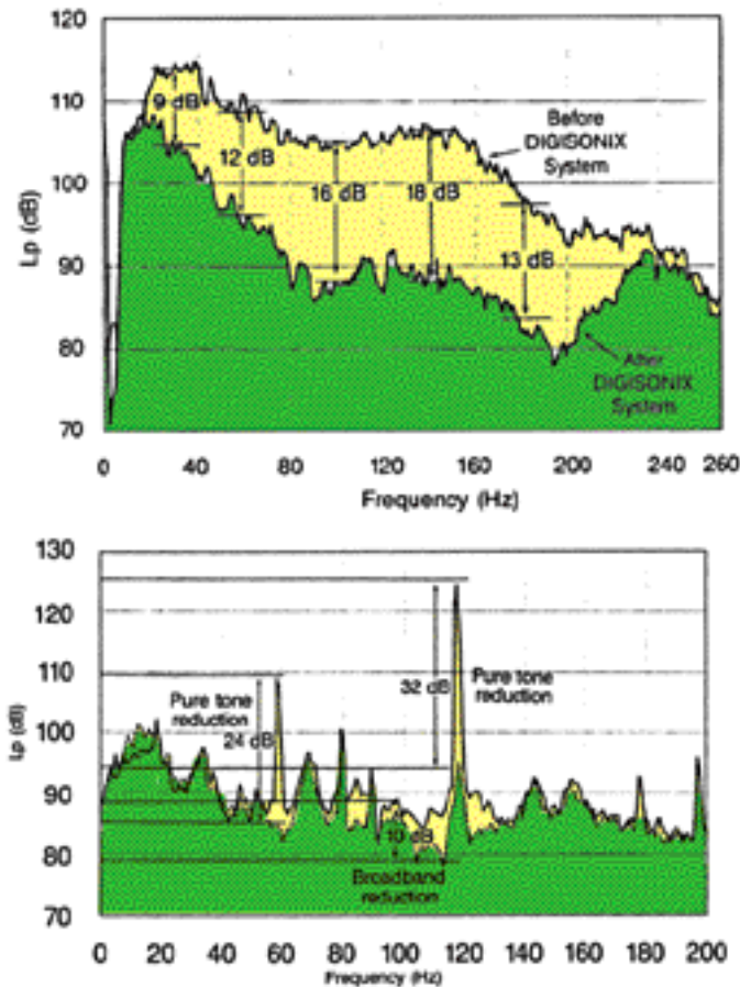
Figure 11: Active noise cancellation efficiency. Traces show power spectrum before (yellow) and after (green) negative feedback, for broadband noise (upper graph) and individual tones (lower graph) (from Eargle 1995).
