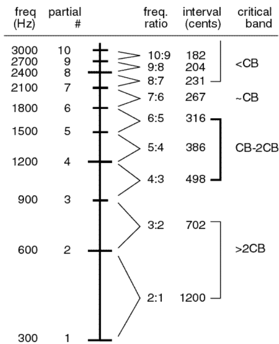
Figure 4: Harmonics 3-5 fall between one and two critical bands (from Braun 1999).
