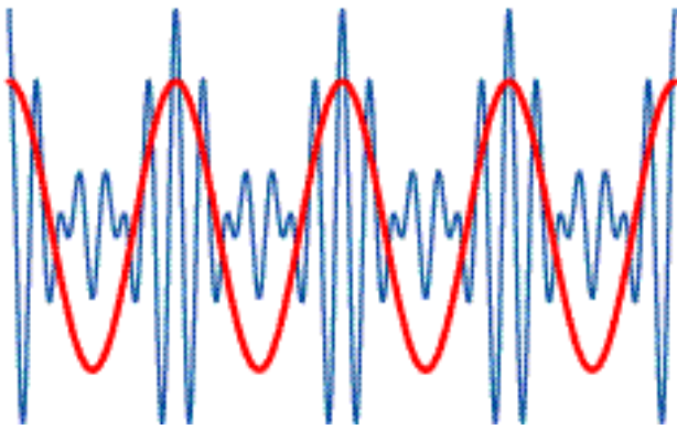
Figure 2: a wave composed only of harmonics 5–7 (blue) has the same periodicity as their fundamental (red) but no spectral energy at the fundamental frequency.
