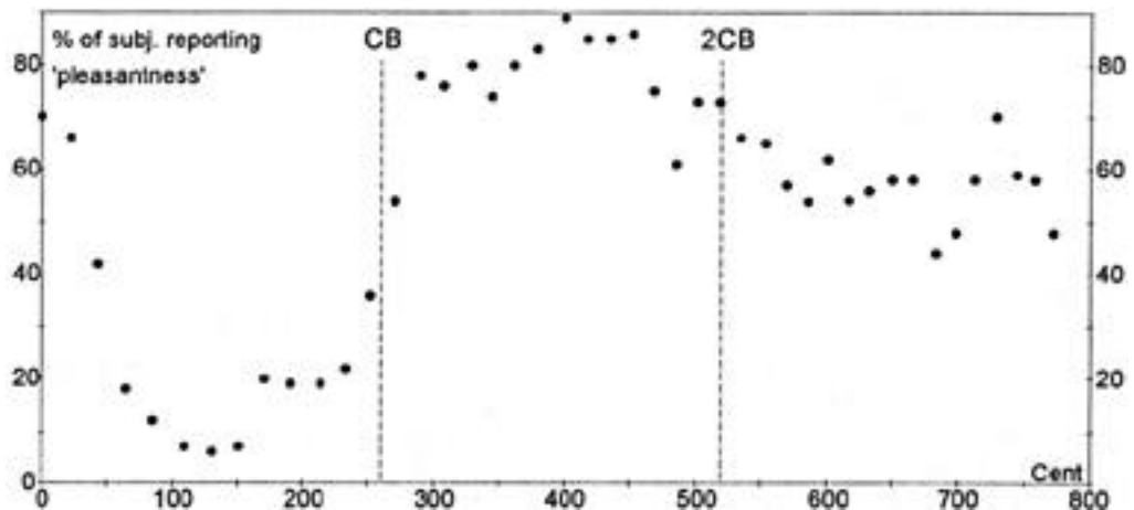
Figure 3: Compiled data of psychophysical percepts as a function of interval size (in cents, which is a logarithmic measure of frequency ratio r : cents = 1200 \log_2 r ). Note here the vertical lines demarcating pitches' trends toward unpleasant for intervals less than one critical band (CB = 260 cents), neutral for those larger than two critical bands (2CB), and pleasant for those between one and two critical bands (from Braun 1999).
