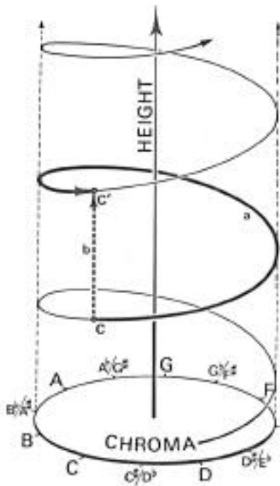
Figure 1: Pitch has been represented as a curve in two dimensions called pitch height and pitch chroma. Height ranges from low, like a thundering rumble, to high, like a shrill birdcall. Chroma represents the musical function of a pitch; in essence, chroma is pitch that has been normalized to a single octave, by assuming all-octave equivalence (from Shepard 1964).
