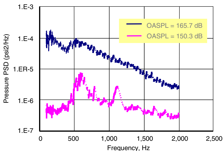
Figure 4. Incident Sonic Spectrum, With and Without Stores
