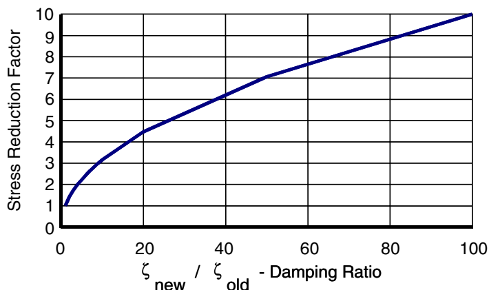
Figure 6. The Effect of Damping on Single Mode RMS Response
