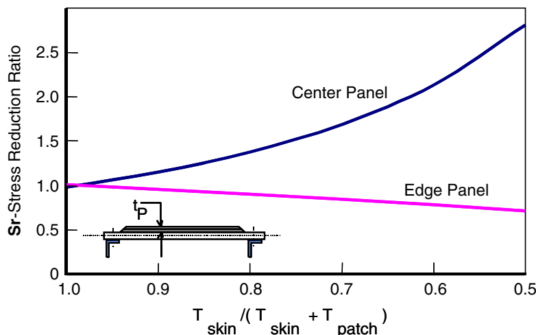
Figure 5. The Effect of Skin Reinforcement on RMS Panel Response
