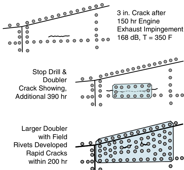
Figure 2. Failed Traditional Sonic Fatigue Repairs
