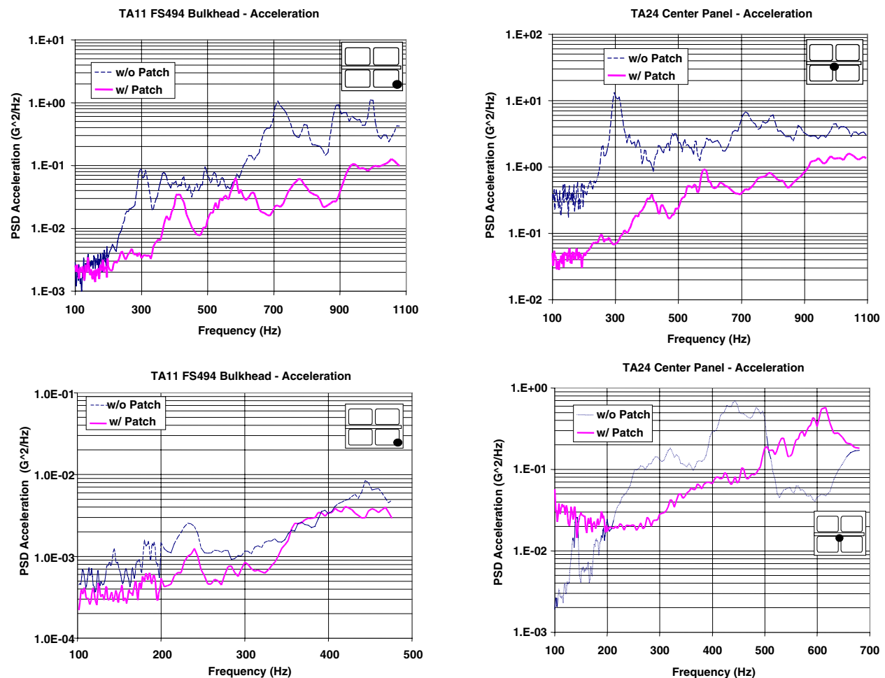
Figure 11. Comparison of Acceleration PSDs w/ and w/o Patch
