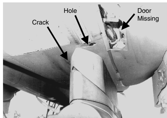
Figure 3. Sonic Damage After Prolonged High Q Flight
