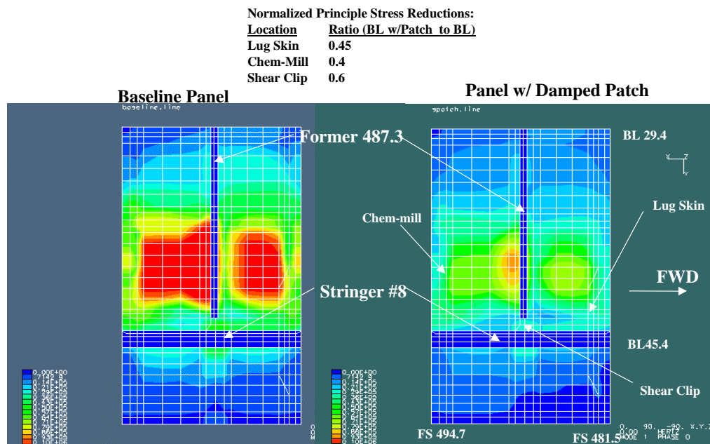
Figure 9. Random Vibration Analysis of Panel with and without Patch
