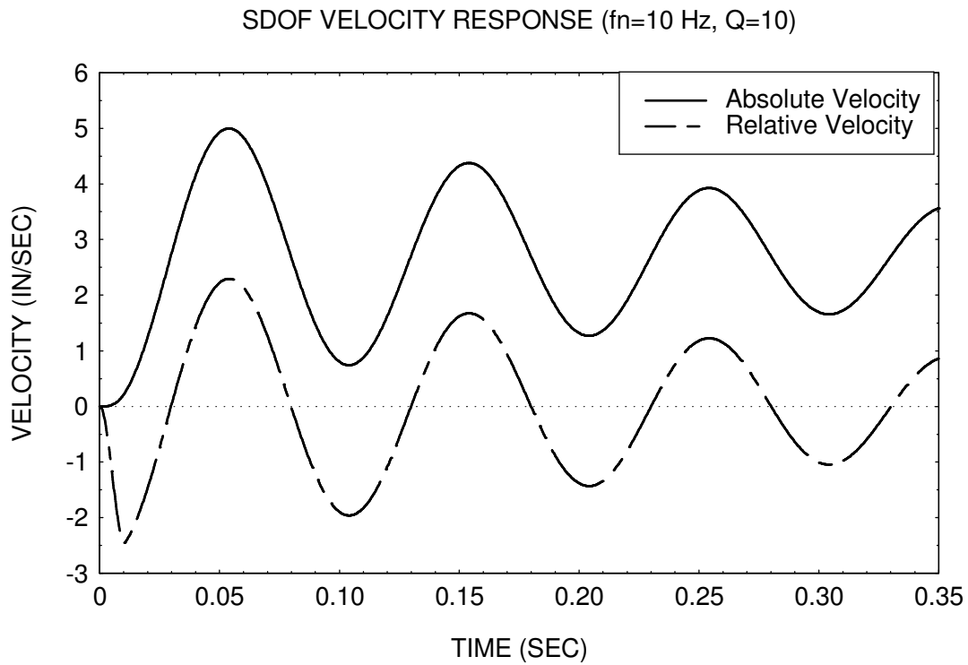
Figure 11. Velocity Response to Half-Sine Pulse
