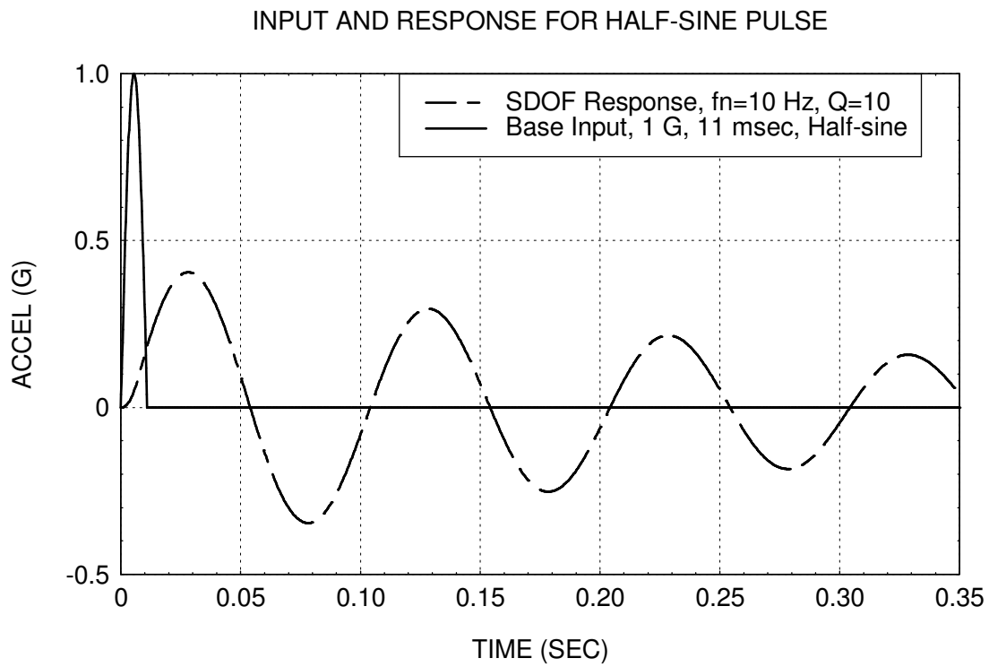
Figure 10. Half-Sine Base Input and Acceleration Response
