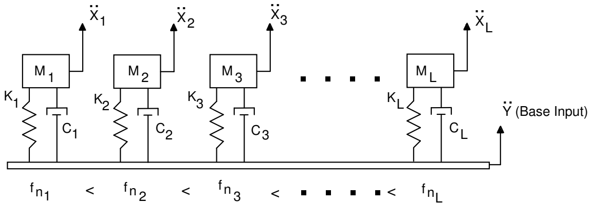
Figure 3. Shock Response Spectrum Model
