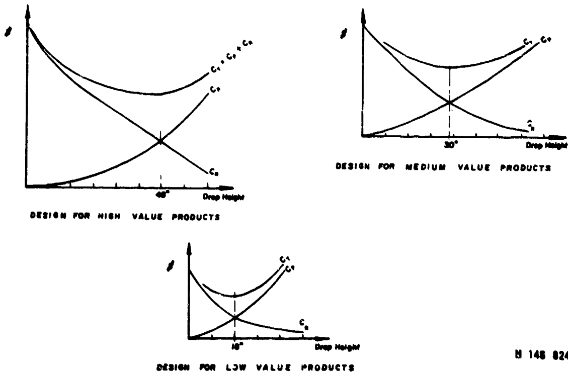
Figure 20.--Package cost versus design drop height for high, medium, and low value products.
