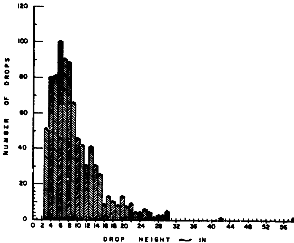
Figure 3.--Drop height versus number of drops (43-lb. container).
