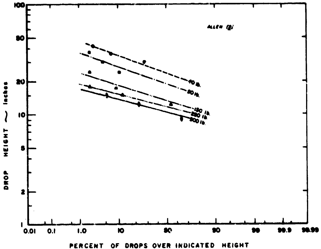
Figure 2.--Drop height versus probability of occurrence (European Studies) (Allen (2)).
