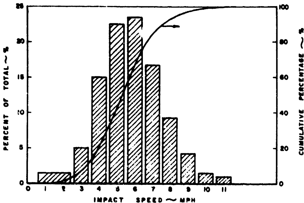
Figure 16.--Distribution of impact speeds based on 4647 observations (51).
