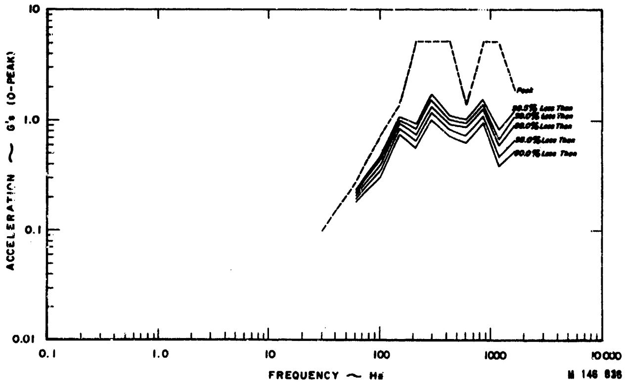
Figure 12.--Frequency spectra for various probabilities--turbojet aircraft (vertical direction, takeoff).
