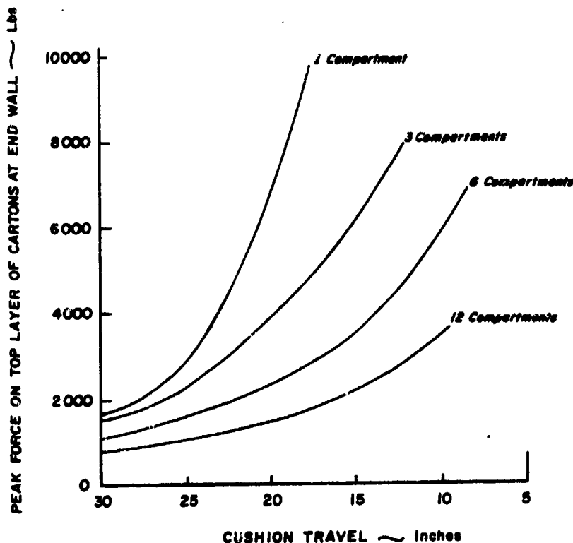
Figure 17.--Effect of compartment on end-wall loading for 10 mile per hour impact.
