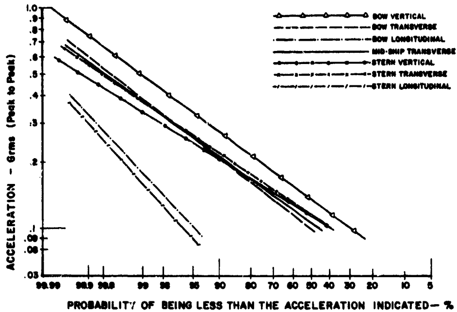
Figure 14.--Wave-induced acceleration versus probability of occurrence (520-ft. cargo ship). M 148 838
