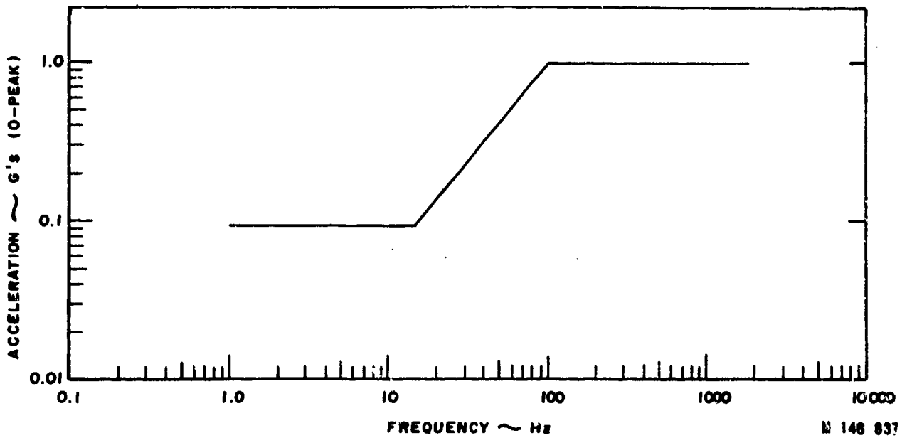
Figure 13.--Acceleration envelope--aircraft.
