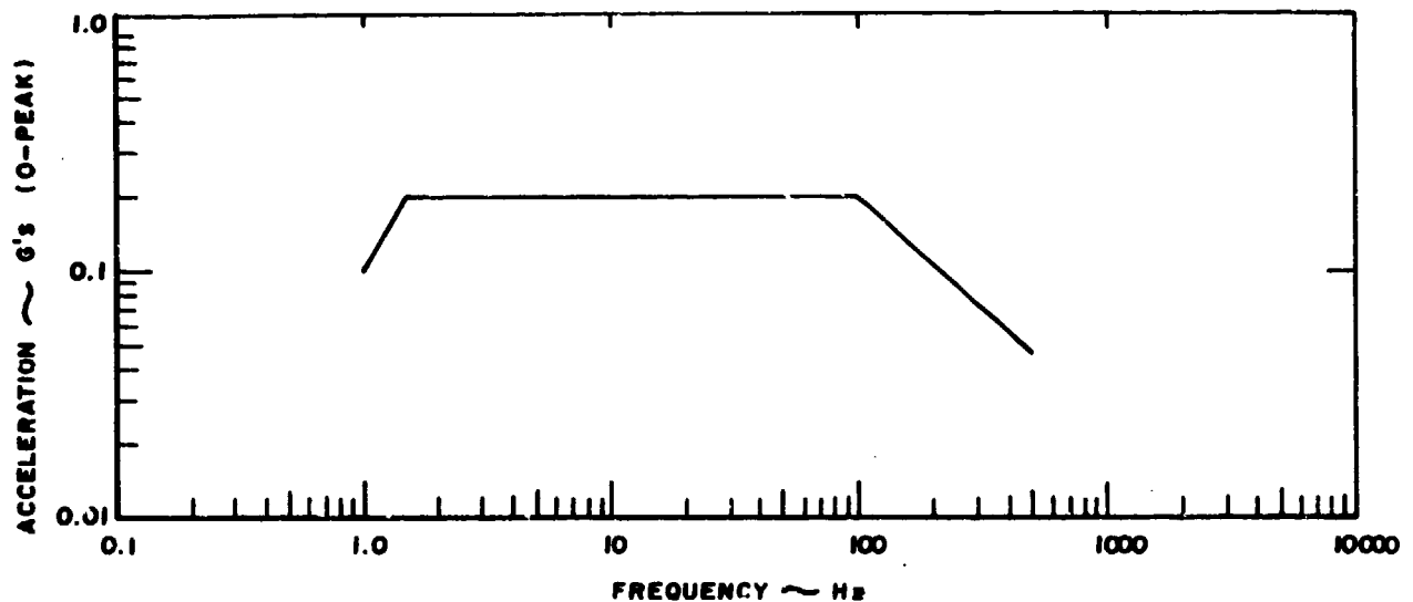
Figure 10.--Vibration acceleration envelope--railcar.
