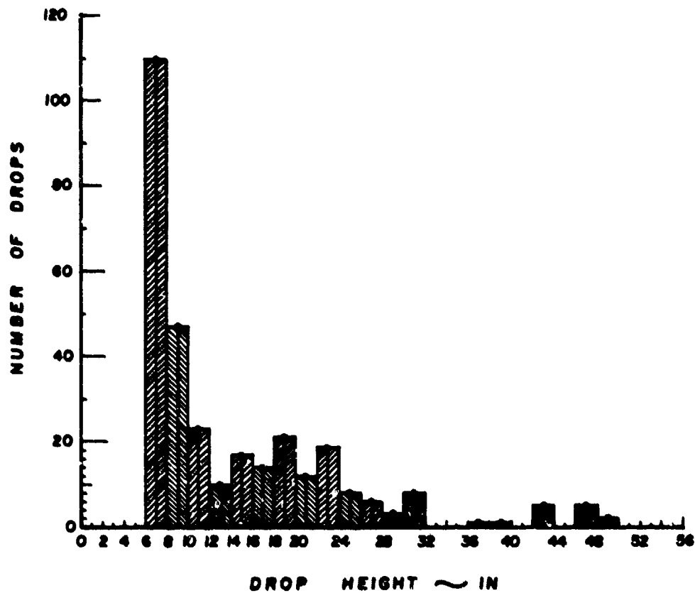
Figure 4.--Drop height versus number of drops (25-lb. container).
