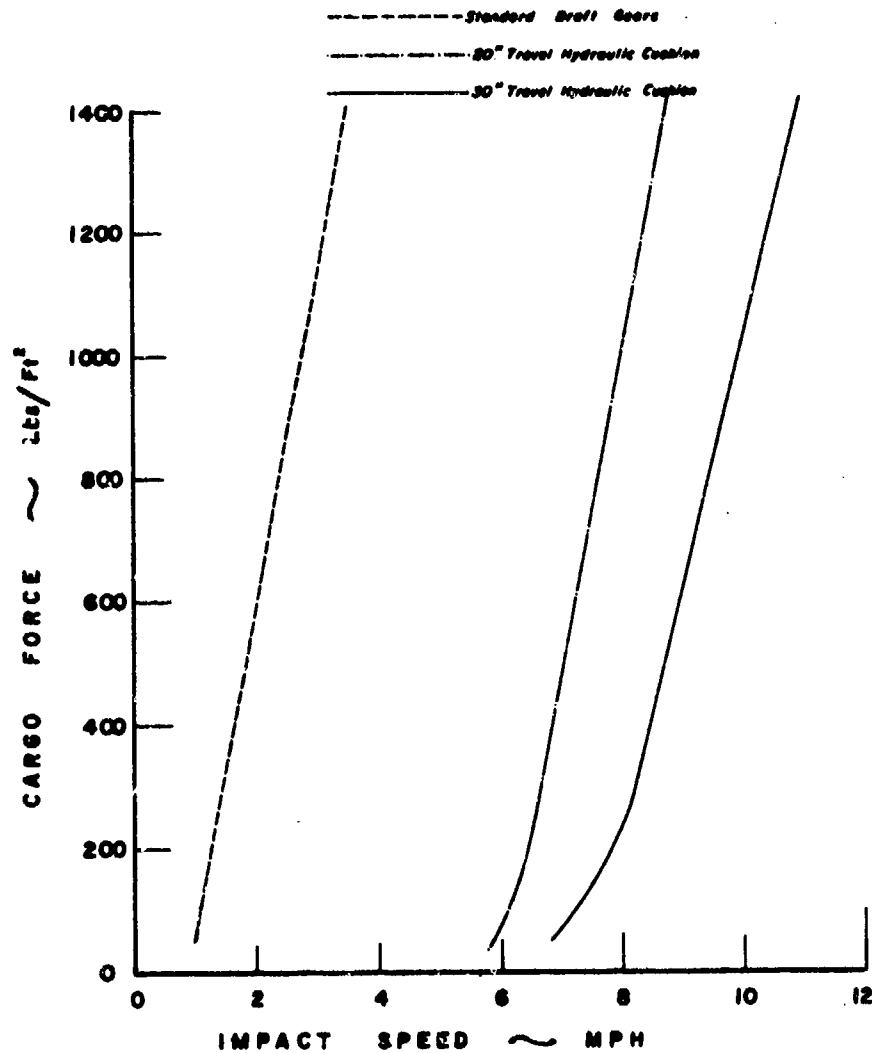
Figure 18.--Cargo force versus impact speed for boxcars having different cushioning systems.
