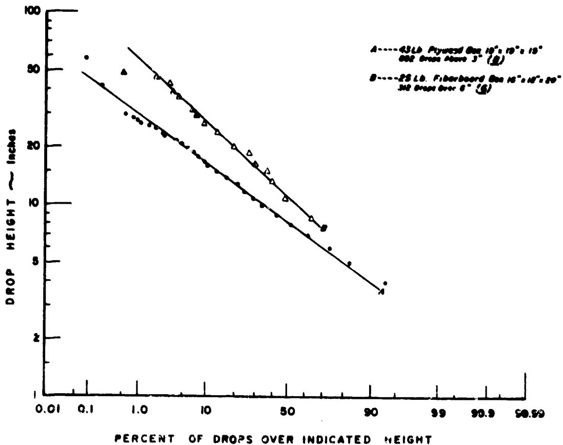
Figure 1.--Drop height versus probability of occurrence (U.S. Studies).
