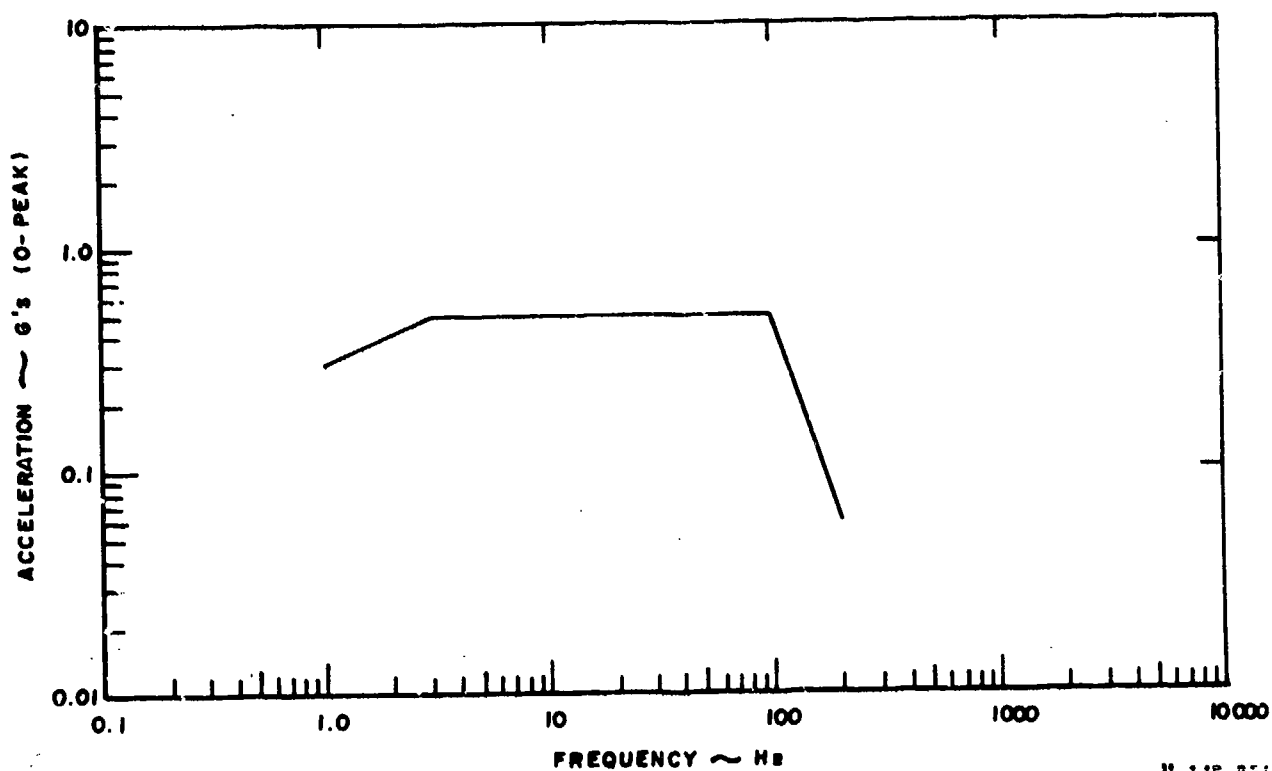
Figure 7.--Vibration envelope curve--truck summary.
