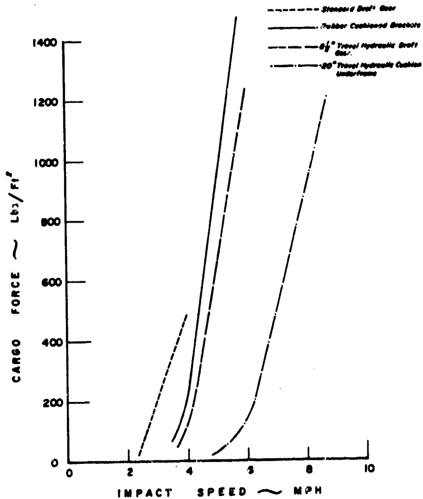
Figure 19.--Cargo force versus impact speed for containers on flatcars (COFC) with different cushioning systems.
