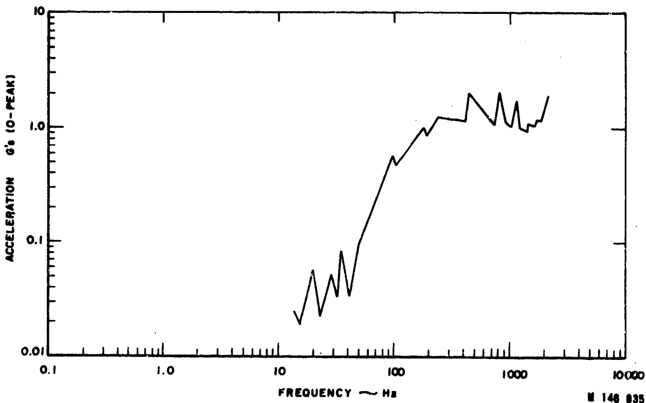
Figure 11.--Aircraft acceleration envelope--turbojet composite.
