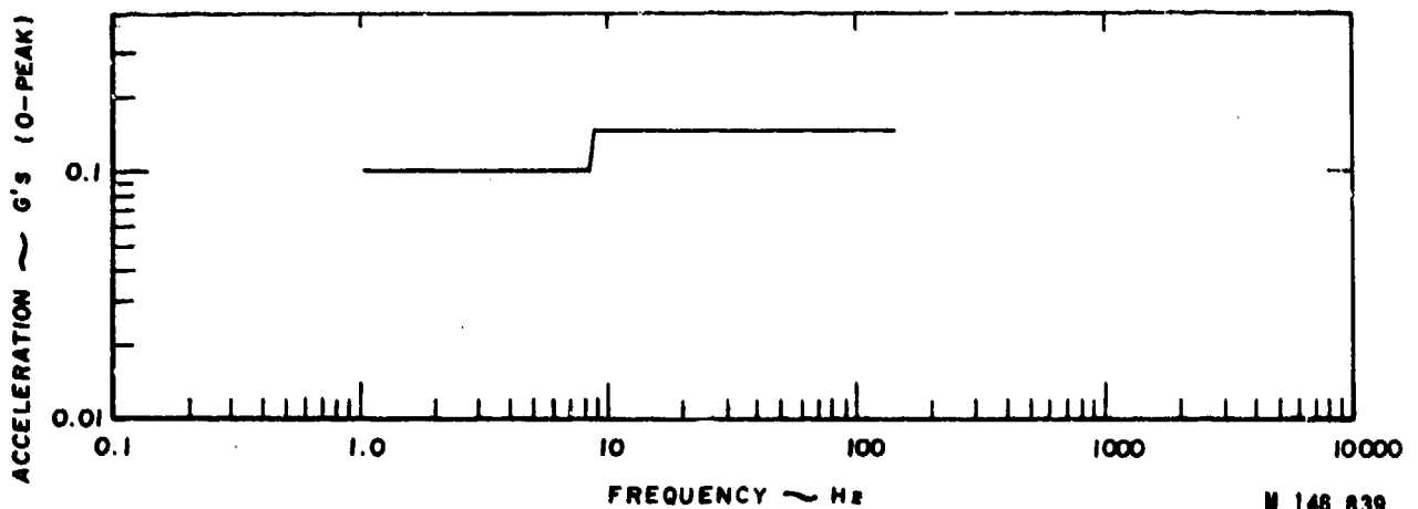
Figure 15.--Vibration spectrum envelope--ship. M 148 839
