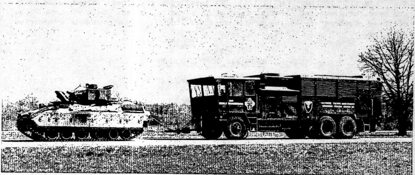
Figure 5. M-2 Infantry Fighting Vehicle undergoing drawbar pull test on dynamometer course.
