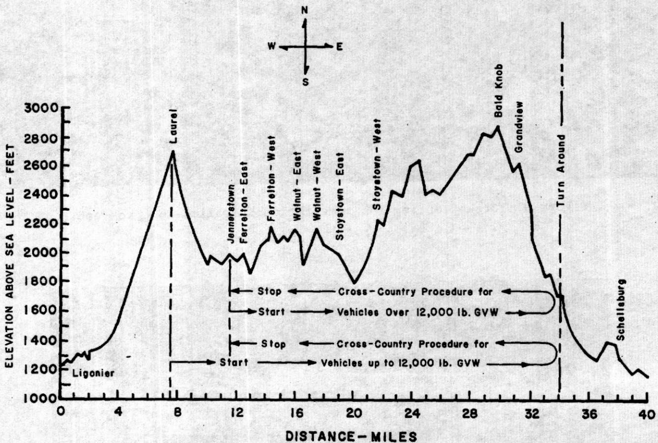
Figure 8. Profile of mountain test course.
