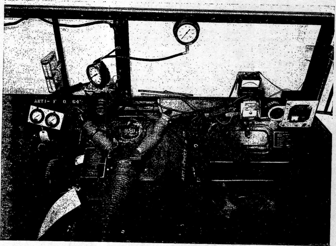
Figure 9. Brake testing instrumentation installed in truck cab.
