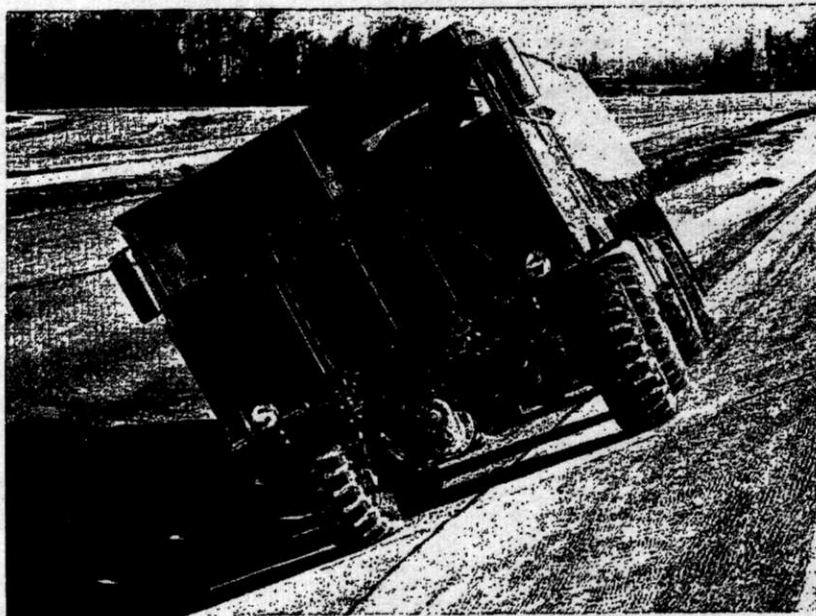
Figure 36. The 40-percent side slope in the Munson area.
