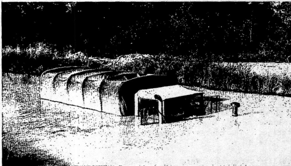
Figure 70. Vehicle in deep water fording facility.
