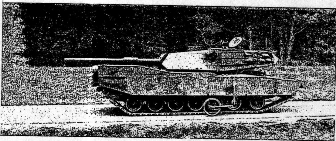
Figure 10. Fifth wheel attached to M-1 for brake test.
