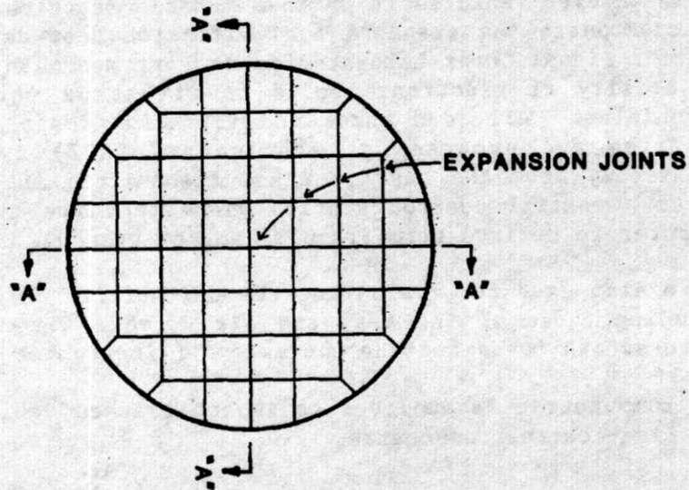
Figure 59. Section and plan view of turning circle.
