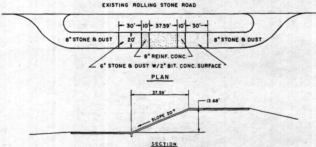
Figure 39. Plan view and section of simulated loading ramp.
