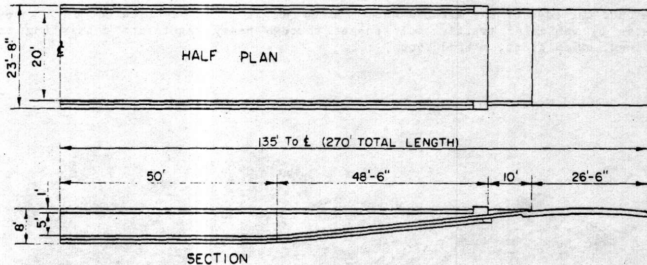
Figure 26. Half plan and section of fording basin.
