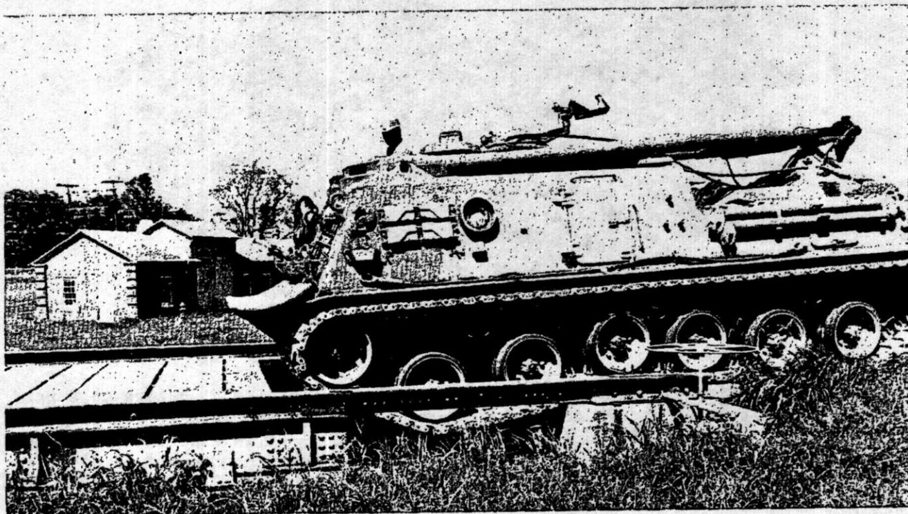
Figure 56. Bridging device.
