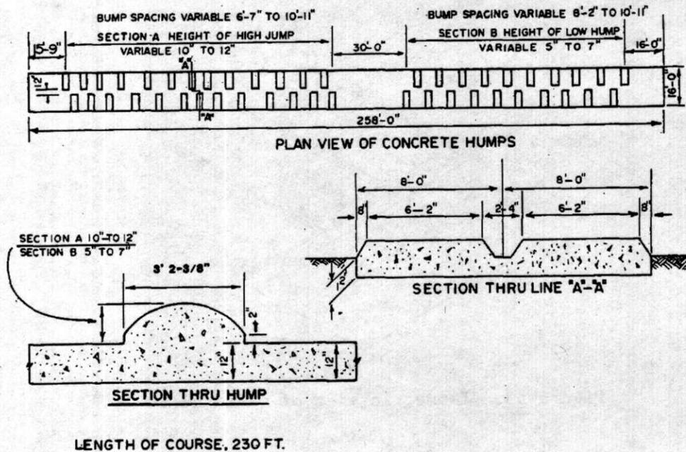
Figure 51. Plan view and sections of staggered bump course.
