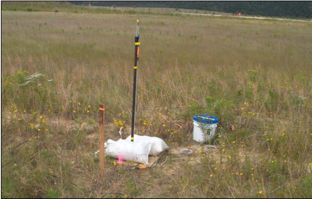
b. 100-m sensor location. Two blast pressure sensors are visible, one mounted on the pipe stand 1.5 m above the ground, and the other on a small metal rod near the ground surface. The white plastic bucket is used to protect the sensor power supplies. Note the tall grass.
