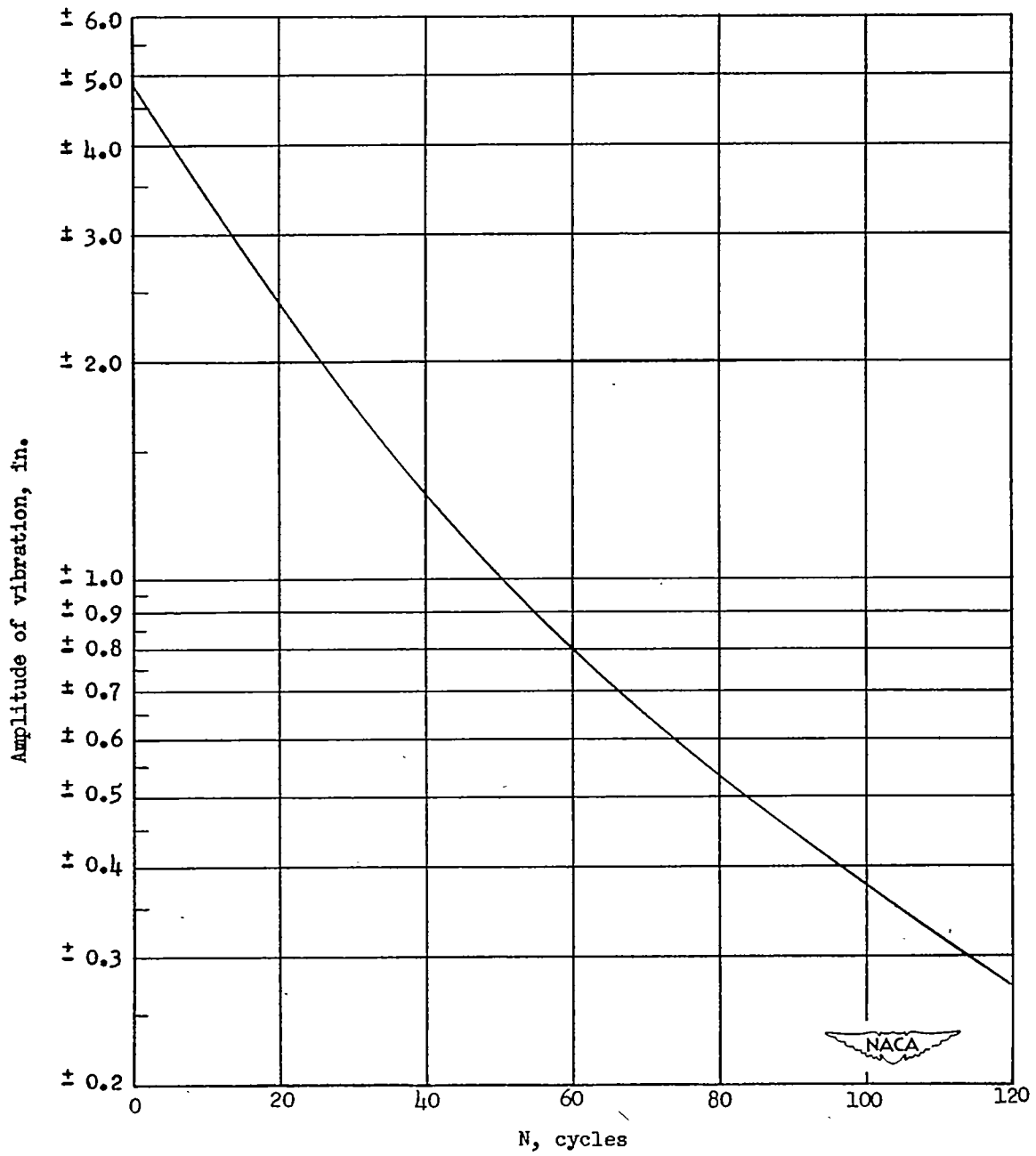
Figure 3.- Decay function of wing for combined data.
