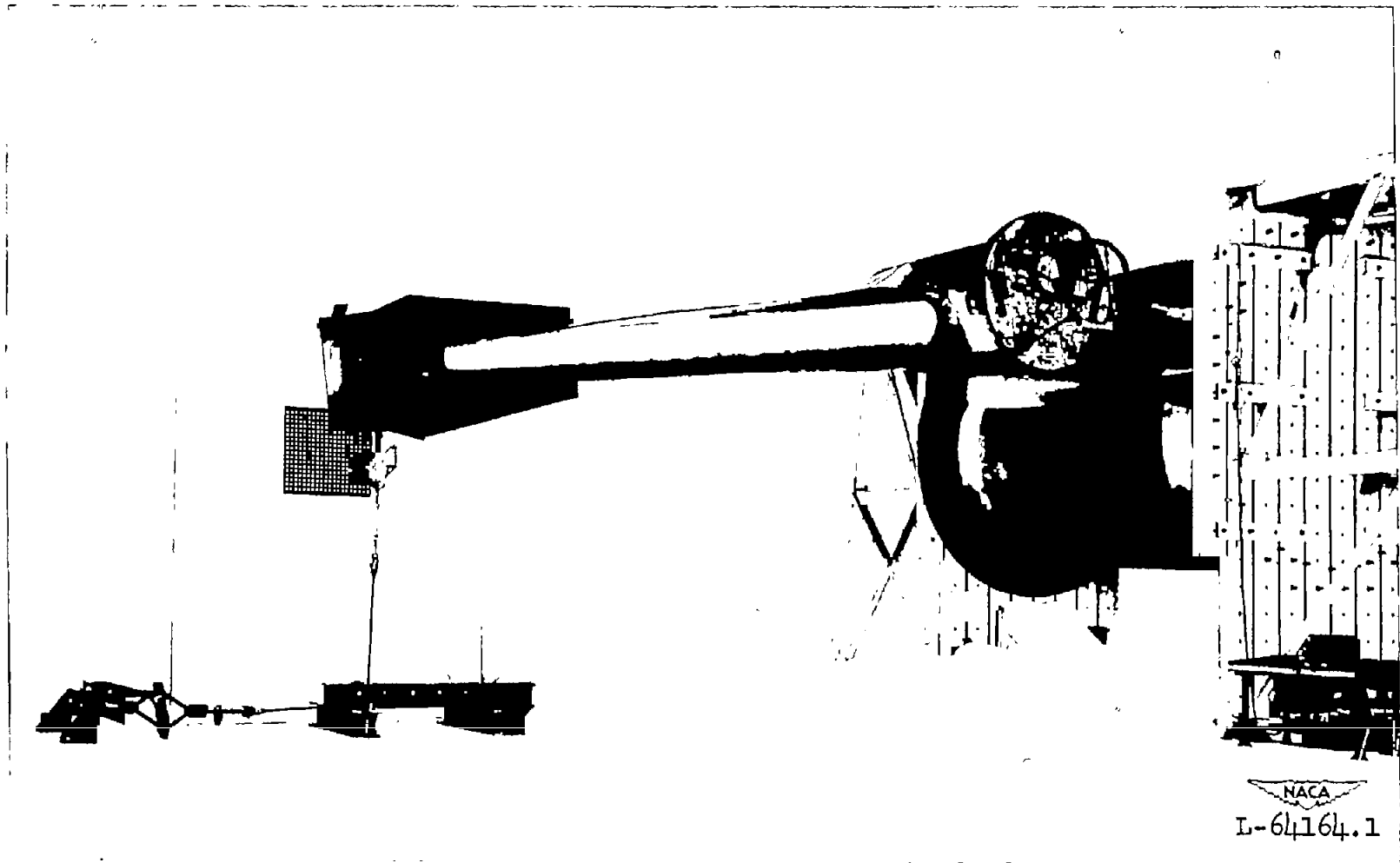
Figure 1.- General view of left half of test setup.
