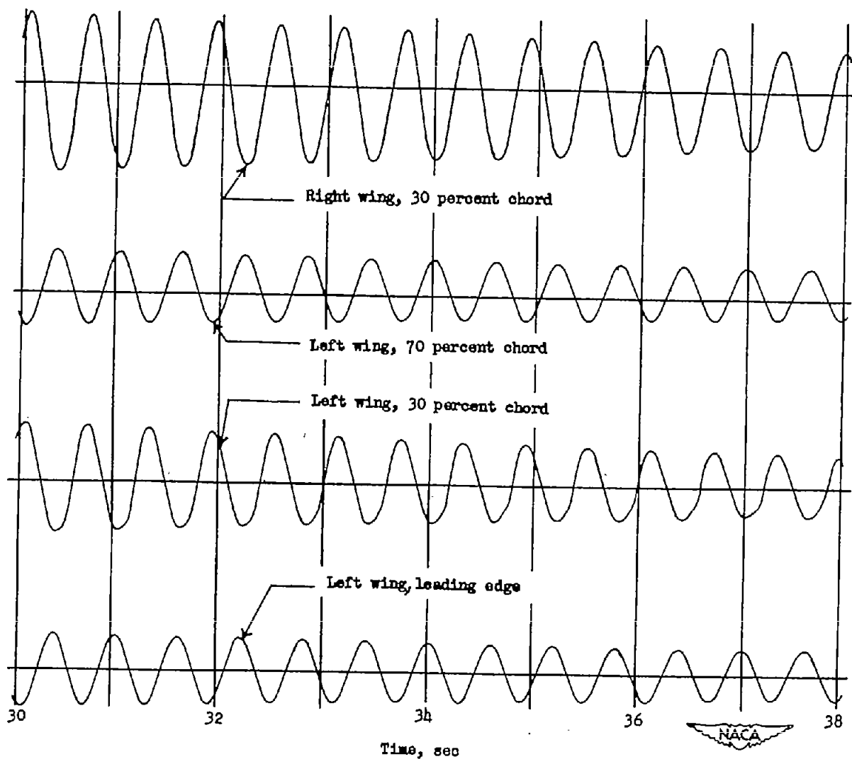
Figure 2.- Sample of vibration time-history record for four accelerometers.
