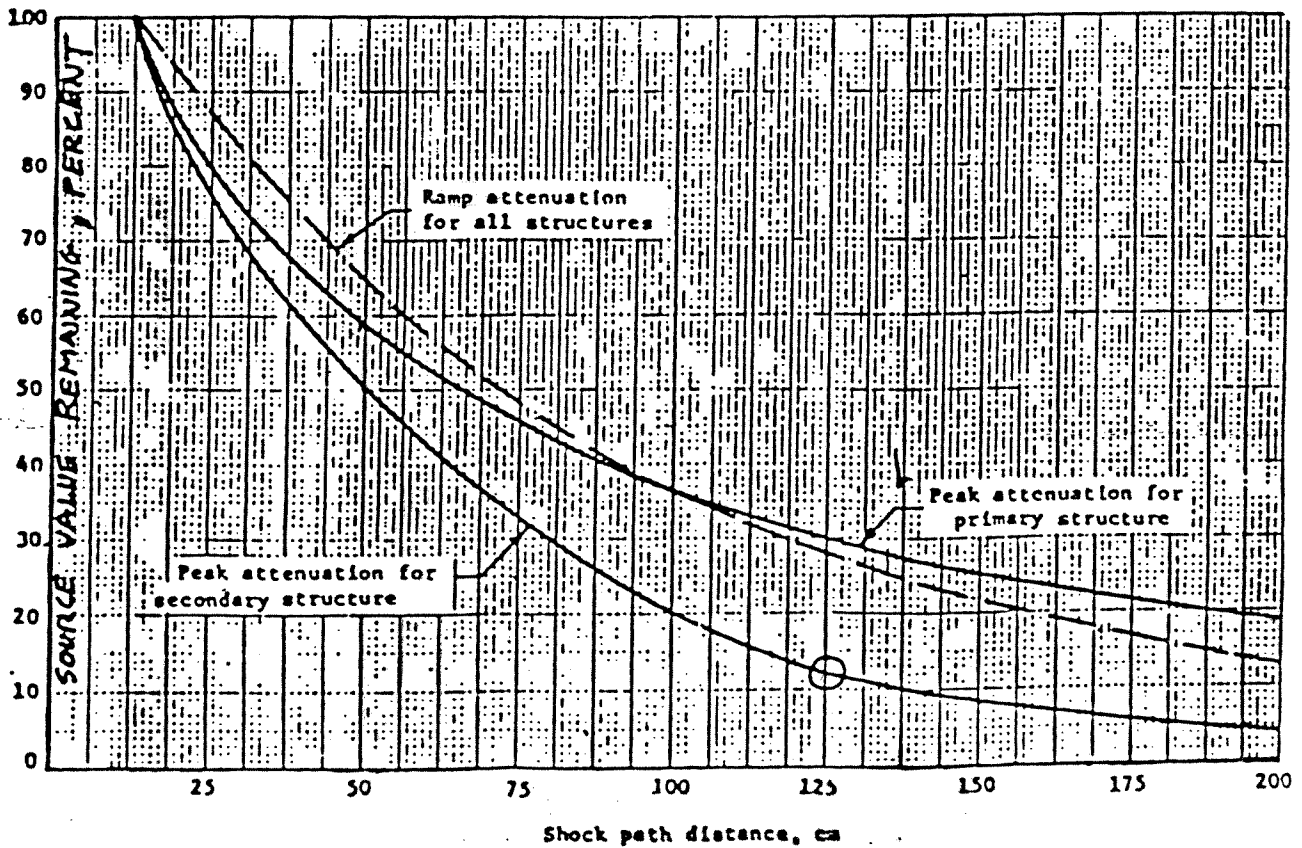
FIGURE 5.2-2. DISTANCE ATTENUATION CURVES FOR PYROTECHNIC SHOCK
