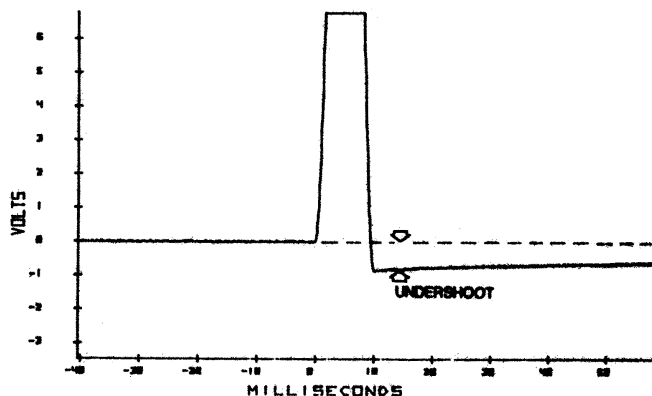
FIGURE 8 ZEROSHIFT DUE TO OVERLOADED ELECTRONICS
